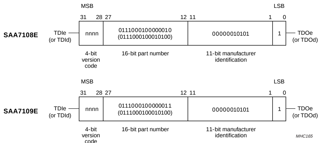
Fig.46 32 bits of identification code.
