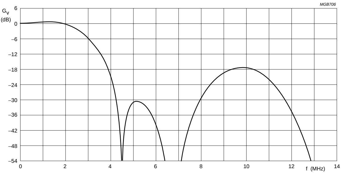
Fig.10 Colour difference transfer characteristic in RGB (excluding scaler).
