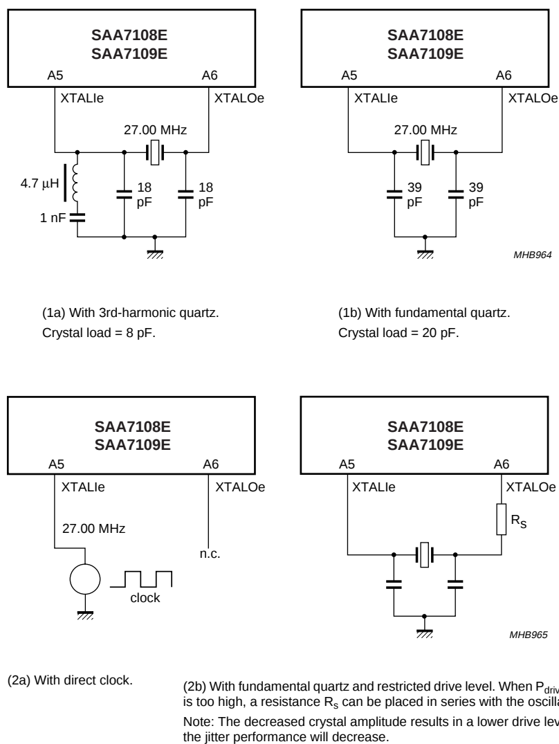
Fig.55 Oscillator application for encoder part.
