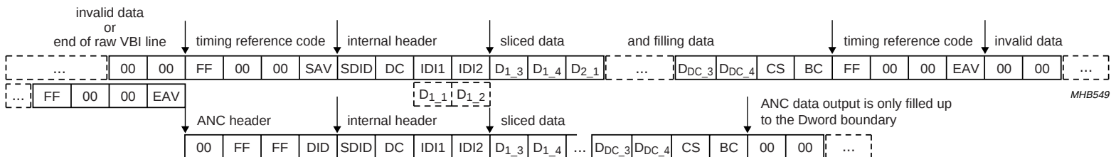
Fig.38 Sliced data formats on the I port in 8-bit mode.
