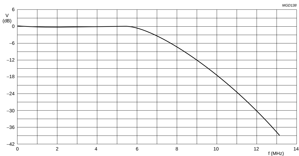
Fig.11 Anti-alias filter.
