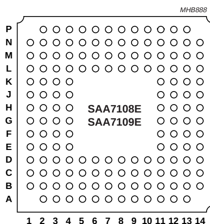
Fig.4 Pin configuration.
